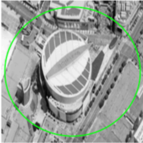
(a) Initialization
