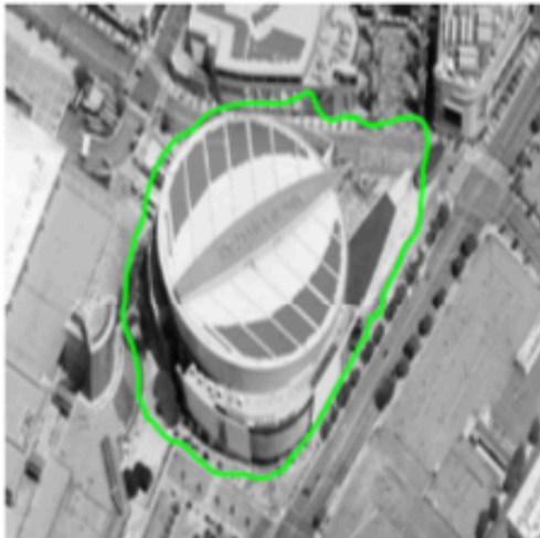
(c) Evolving
