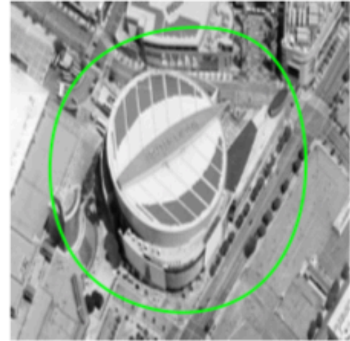
(b) Evolving
